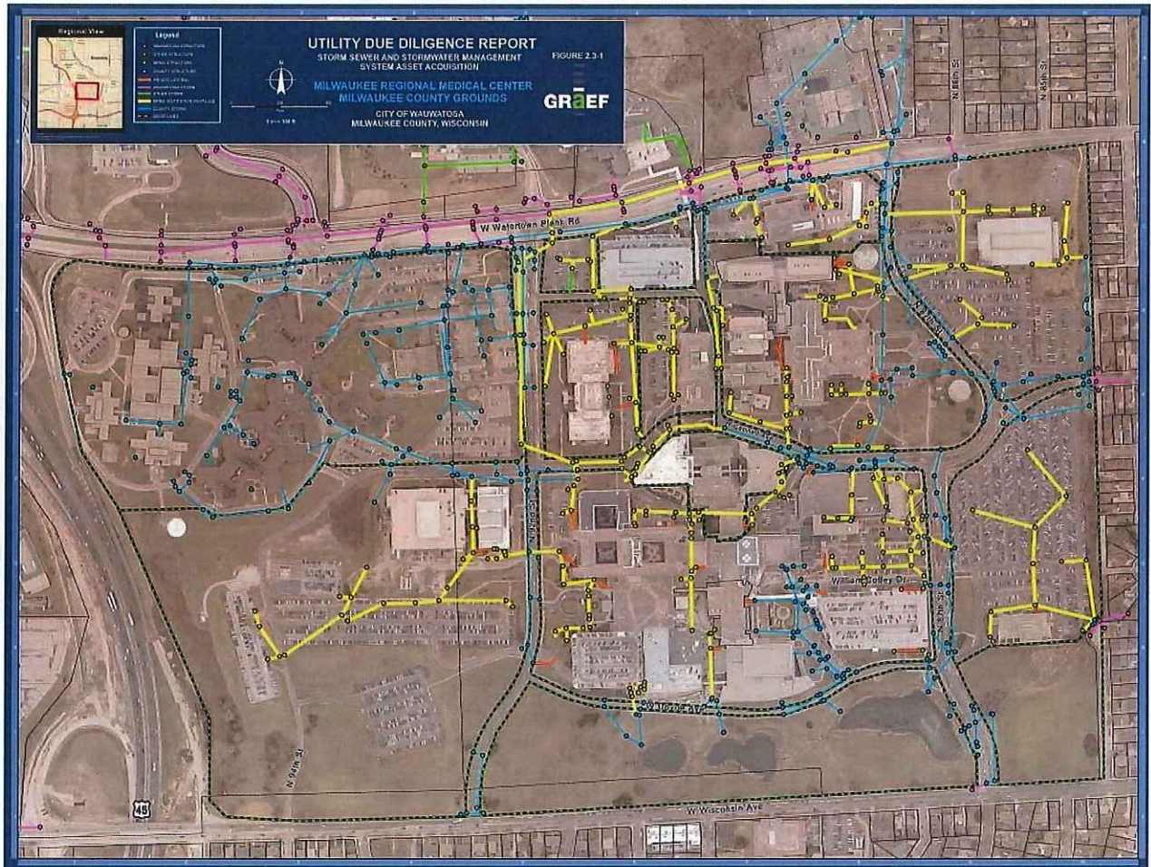
Figure B-2 Storm Sewer Main
