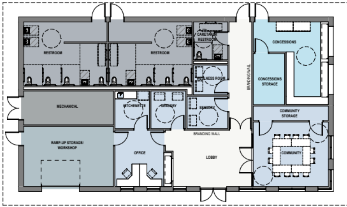
1 1ST FLOOR PLAN 1/8" = 1'-0"
