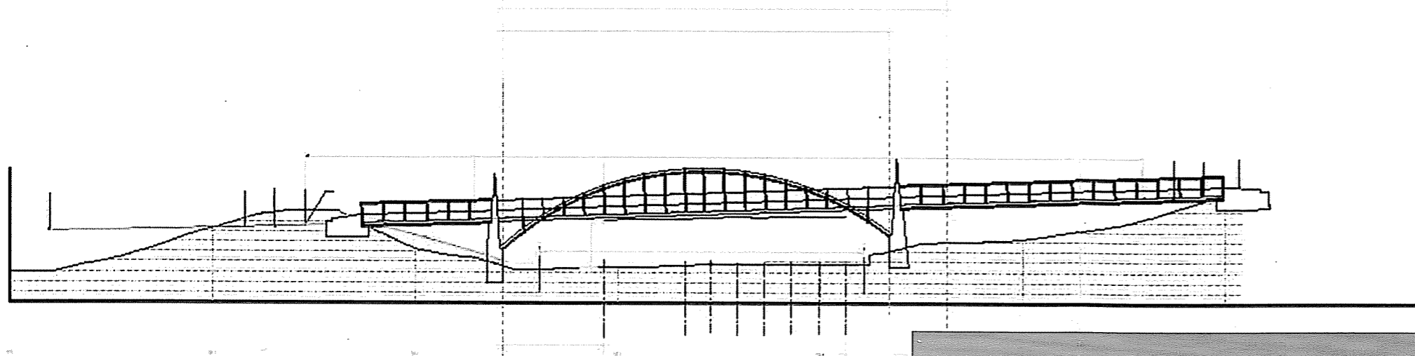
PROFILE - 3 SPAN WITH ARCH
